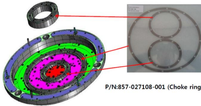
Gasket on TCP (Upper Side)
