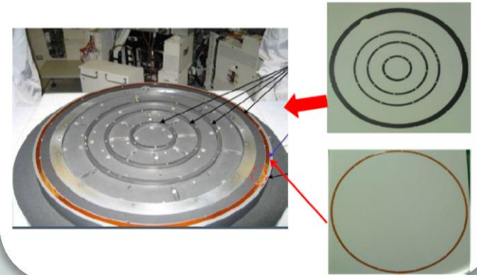
Gasket on TCP (Upper Side)
