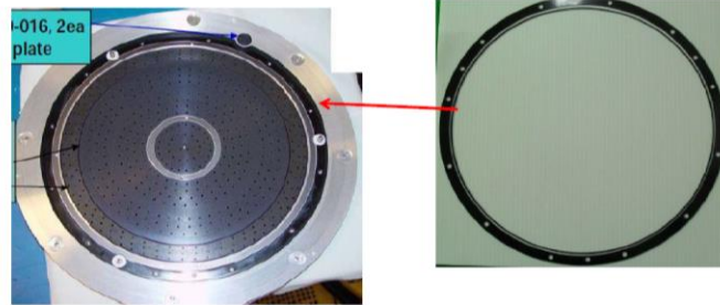
Gasket on Backing Plate (Low Side)
