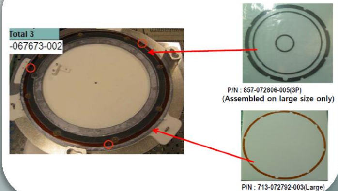
Gasket on Outer Cathode
