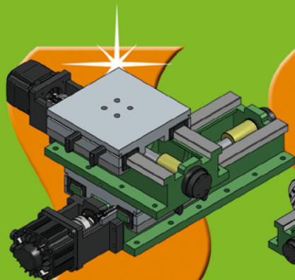
XY 伺服硬軌滑台 XY Servo Headness Slide Unit
