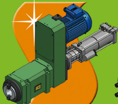
搪銑主軸頭 / 氣動打刀缸 Boring / Milling Head Unit / with Unclamping Cylinder
