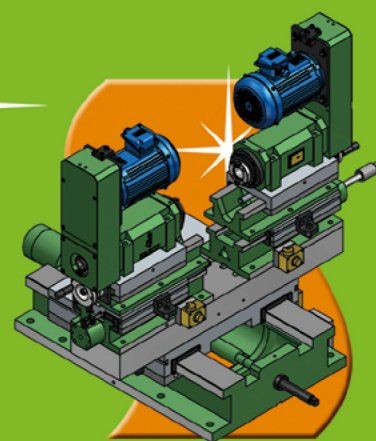
XY 液壓滑台+搪銑頭 XY Hydraulic Slide + Milling Head
